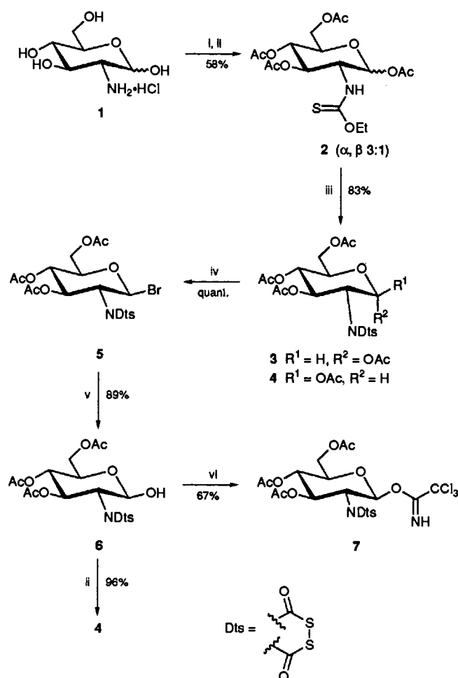
Scheme 1 Reagents: i, EtOC(S)SCH 2 CO 2 H, MeOH; ii, Ac 2 O, pyridine; iii, ClC(S)OCl, CH 2 Cl 2 ; iv, 33% HBr, HOAc; v, aq. acetone; vi, CCl 3 CN, K 2 CO 3 , CH 2 Cl 2
