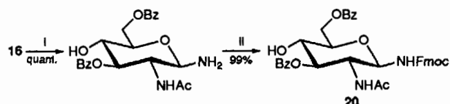
Scheme 5 Reagents: i, H 2 , Pd/C; ii, Fmoc-OSu, pyridine
