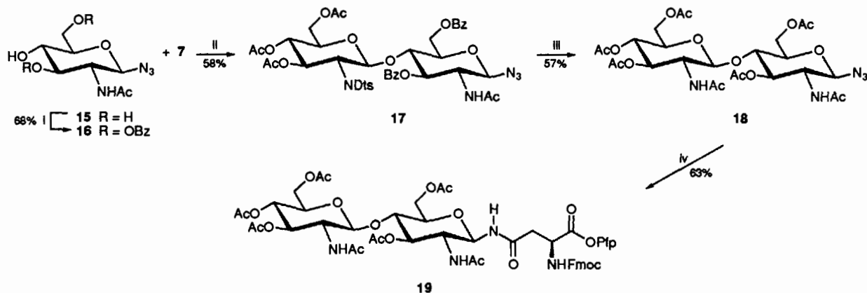
Scheme 4 Reagents: i, BzCl, pyridine, CH 2 Cl 2 ; ii, TMSOTf, CH 2 Cl 2 ; iii, (a) NaBH 4 , CH 2 Cl 2 -MeOH; (b) Ac 2 O, pyridine; iv, (a) H 2 , Pd/C (10%); (b) Fmoc-Asp(Cl)-OPfp, N -ethylmorpholine, THF
