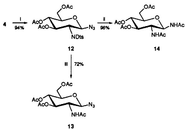
Scheme 3 Reagents: i, TMSN 3 , SnCl 4 , CH 2 Cl 2 ; ii, (a) DTT, CH 2 Cl 2 ; (b) Ac 2 O, pyridine; iii, (a) NaBH 4 , CH 2 Cl 2 , MeOH (1:1); (b) Ac 2 O, pyridine
