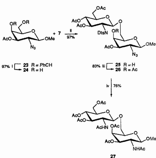
Scheme 7 Reagents and conditions: i, 80% HOAc, 70 °C; ii, TMSOTf, CH 2 Cl 2 ; iii, Ac 2 O, pyridine; iv, DTT, diisopropylethylamine, CH 2 Cl 2 , MeOH; then Ac 2 O, pyridine
